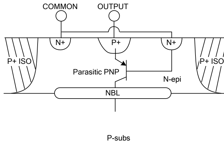
Construction of the Surge-Absorbing Diode
