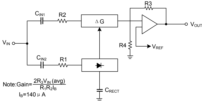
Figure 3. Basic Expander
