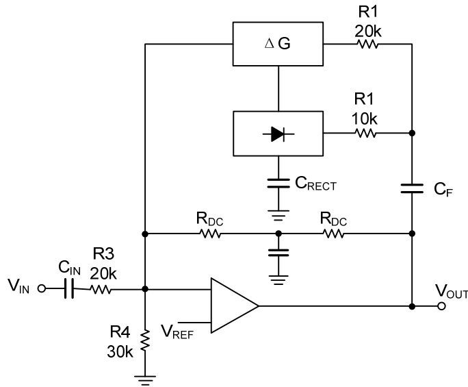
Figure 4.Basic Components
