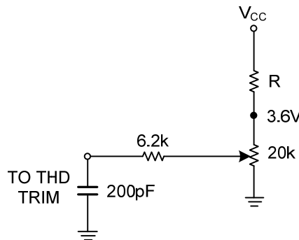
Figure 11. THD Trim Network
