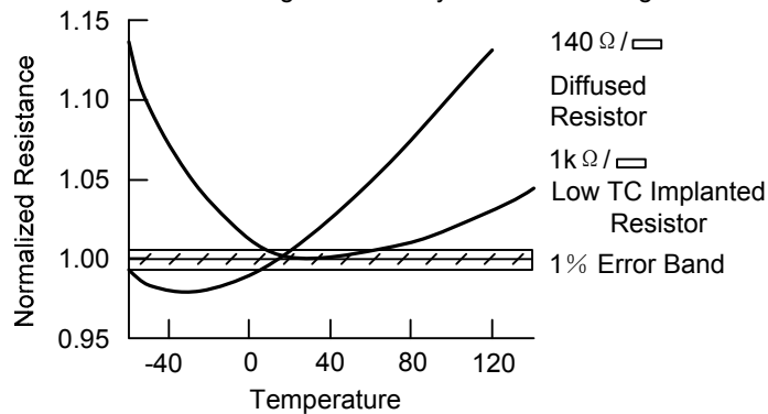
Figure 15.Resistance vs Temperature
