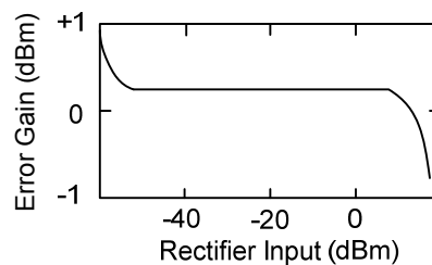
Figure 7.Rectifier Accuracy
