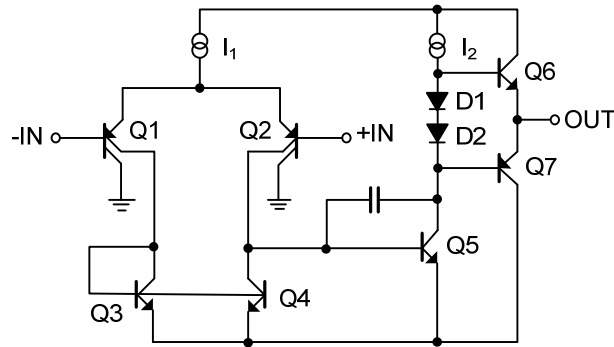
Figure 14.Operational Amplifier
