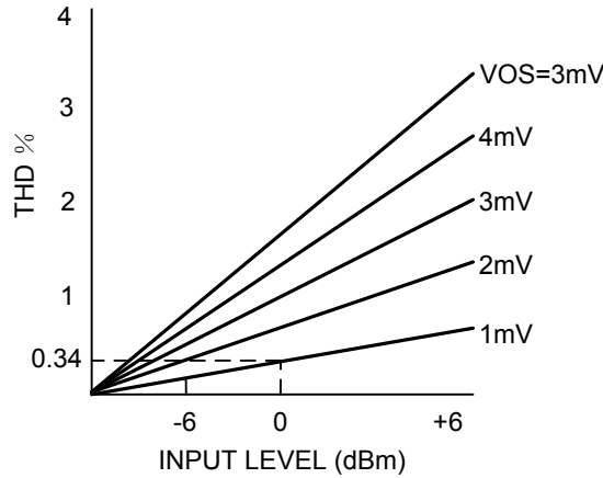
Figure 10.G Cell Distortion vs Offset Voltage
