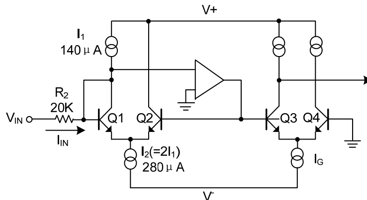
Figure 8.Simplified G Cell Schematic
