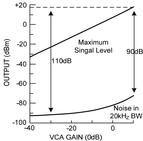
Figure 12.Dynamic Range of UTC571
