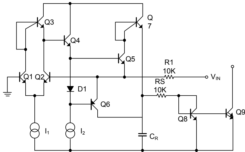
Figure 6.Simplified Rectifier Schematic
