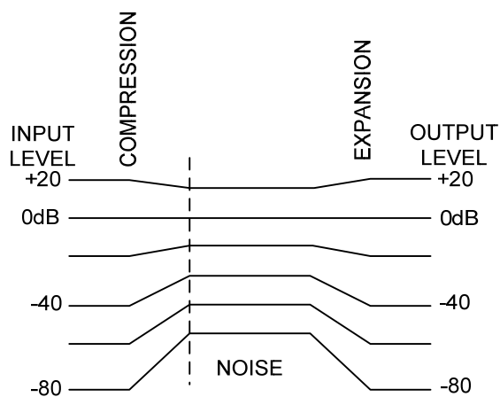
Figure 1. Restricted Dynamic Range Channel
