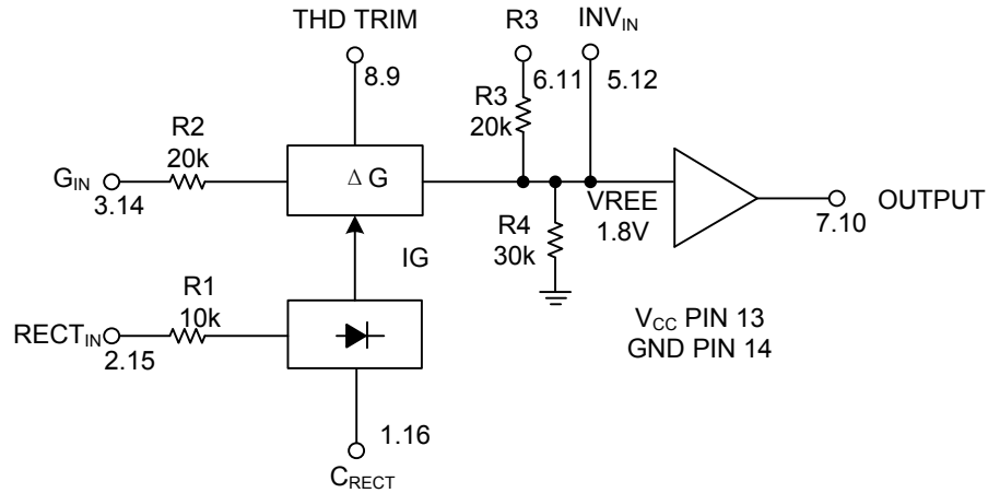
Figure 2. Chip Block Diagram
