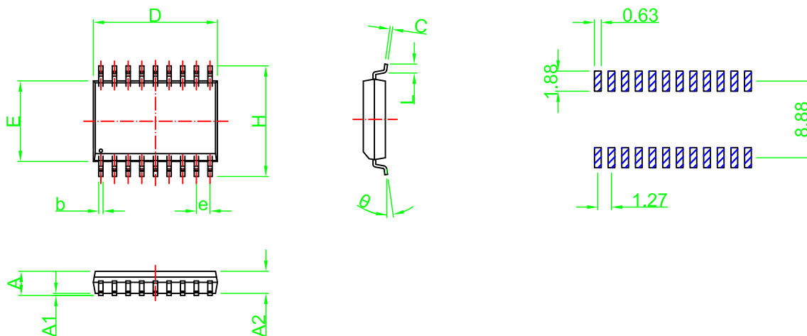
Recommended Land Pattern
