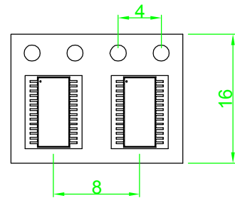
TSSOP-28 T/R
