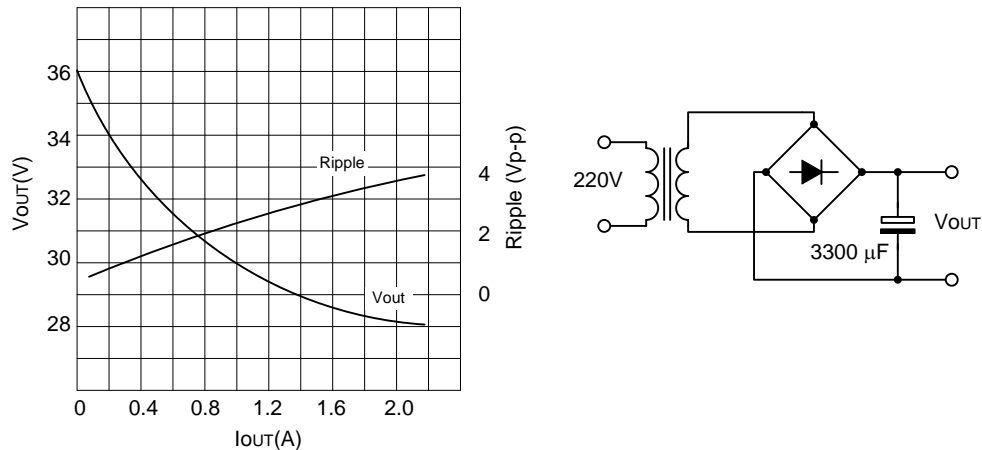
Fig. 10 DC characteristics of 50W non-regulated supply
