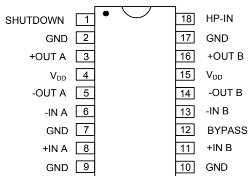
SOP-18
