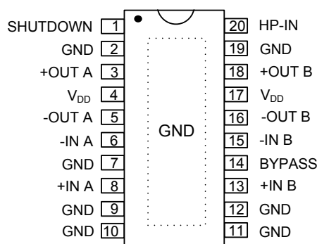
HTSSOP-20 (Top View)
