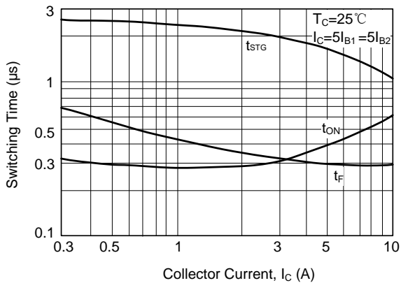
Switching Time
