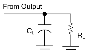
TEST CIRCUIT
