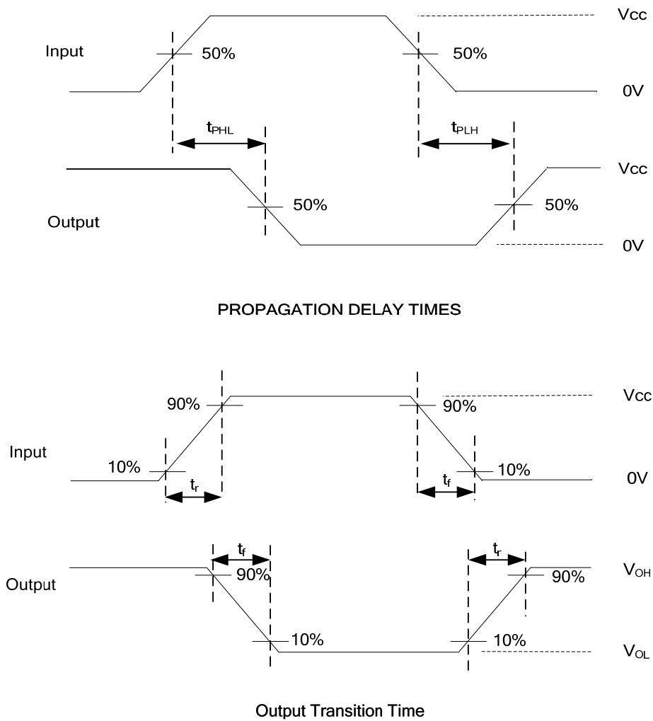
Fig. 2 Propagation delay from input(A) to output(Y) and Output transition time.
