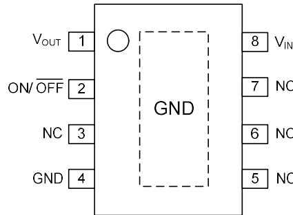
HSOP-8 (Fixed)
