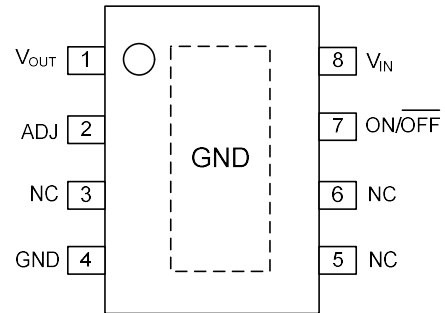
HSOP-8 (Adjustable)
