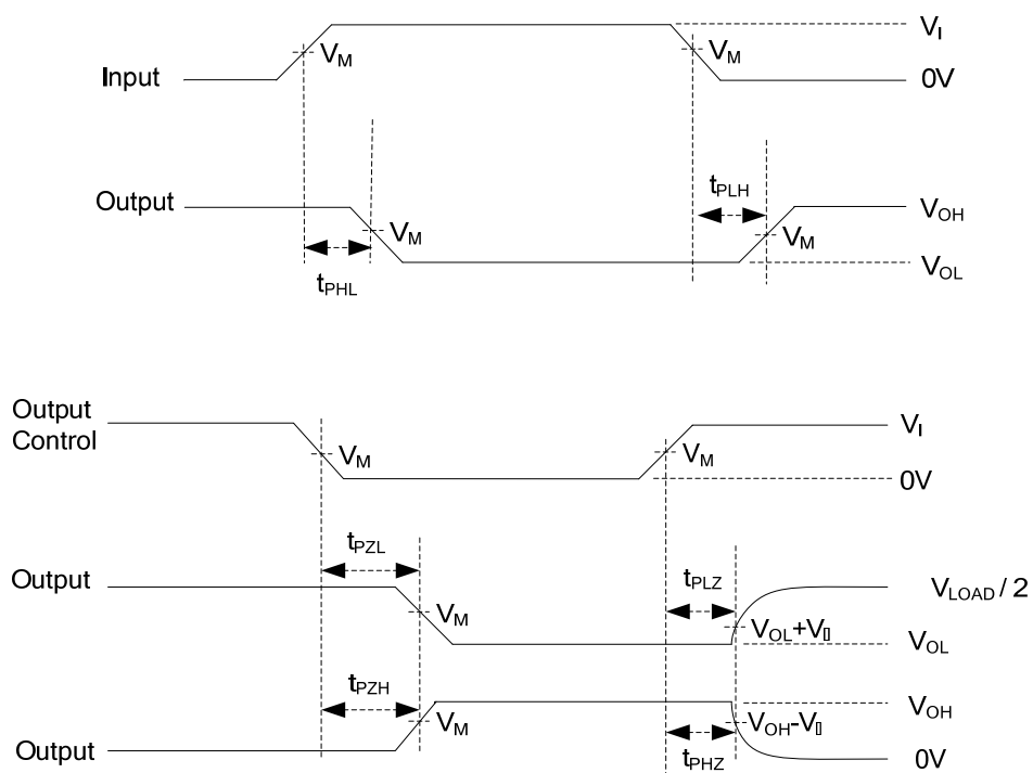
Figure 2. Propagation Delay Waves
