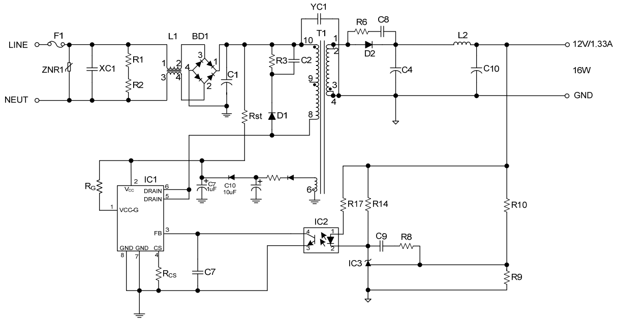
Fig.8 UTC US1602 Typical Application Circuit
