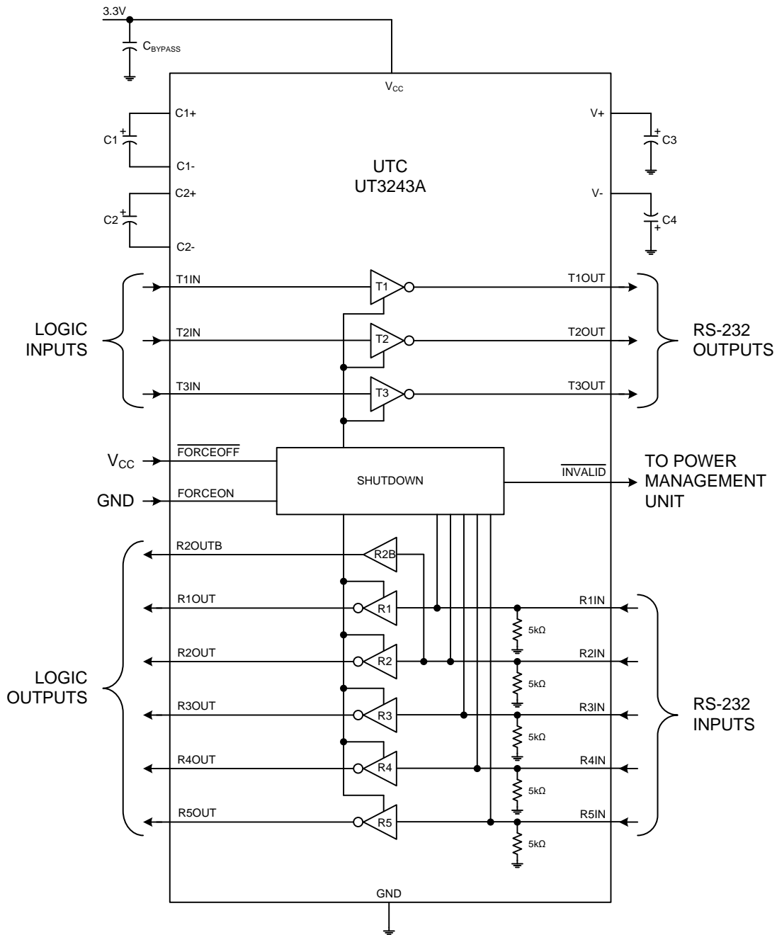
Fig.3 Application Circuit
