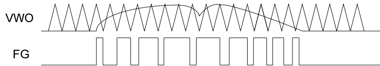
Figure 4. Sinusoidal PWM
