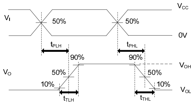
Fig 2. Propagation Delay Times
