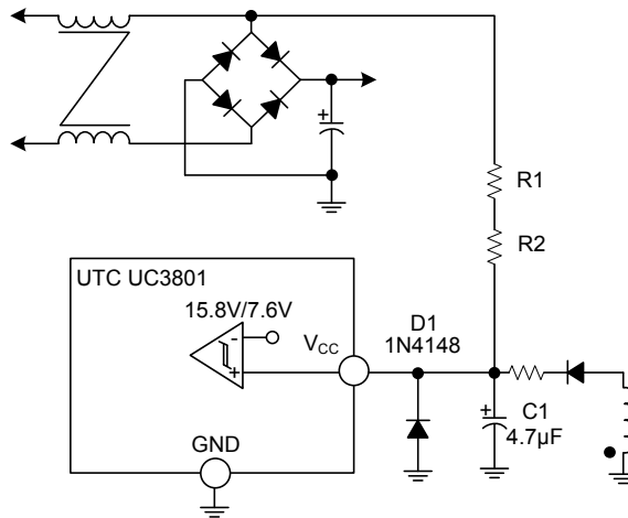
Fig. 1 Startup Circuit
