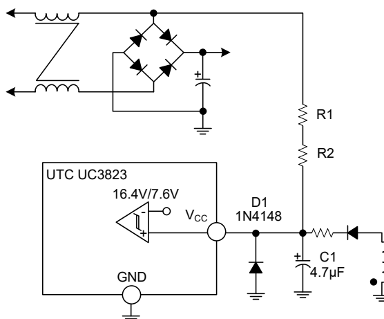
Fig. 1 Startup Circuit
