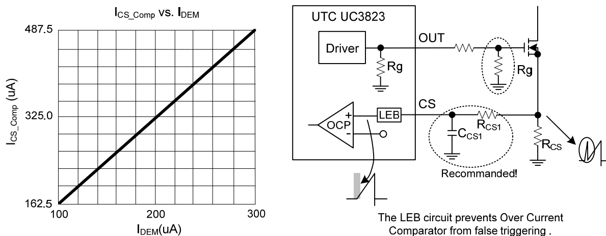
Fig. 7 Current Sensing
