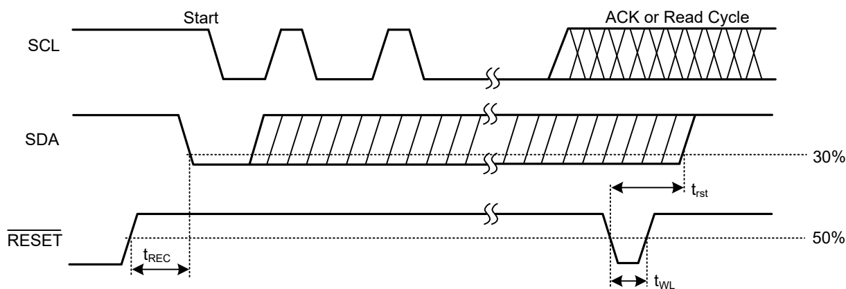
Figure 2. Reset Timing
