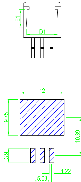
Recommended Land Pattern
