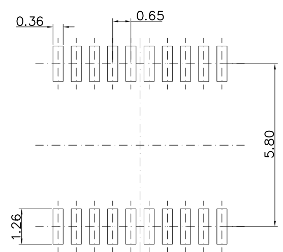
LAND PATTERN
