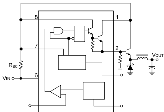
2a. External NPN Switch
