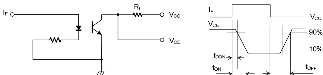
Switchin Time Test Circuit
