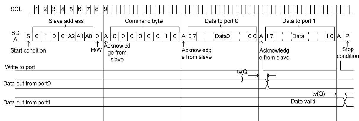
Figure 7. Write to output port registers
