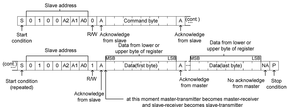
Figure 9. Read from register
