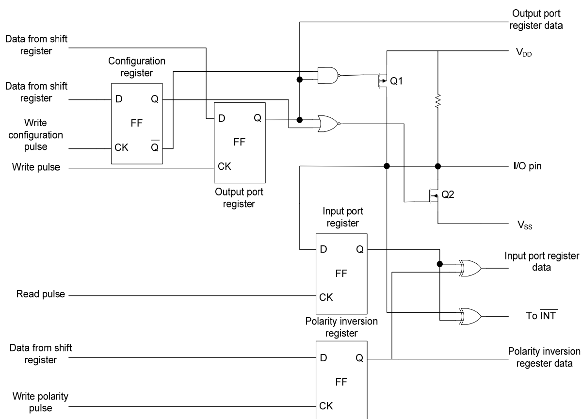
Figure 6. Simplified schematic of I/Os
