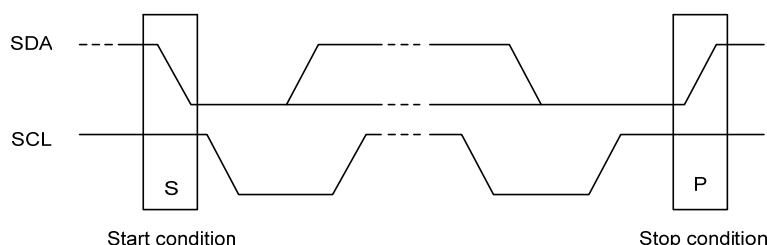
Figure 13. Definition of start and stop conditions
