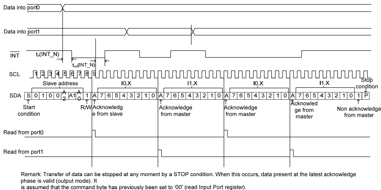
Figure 10. Read input port registers, scenario 1
