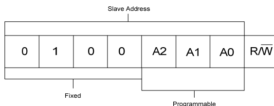
Figure 4. UCA9535 Device Address
