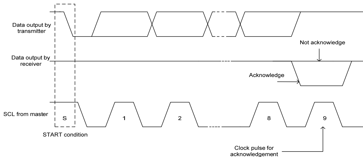
Figure 15. Acknowledgement on the I 2 C-bus
