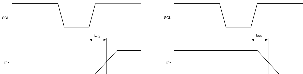
Figure 3. t_{V(O)} timing
