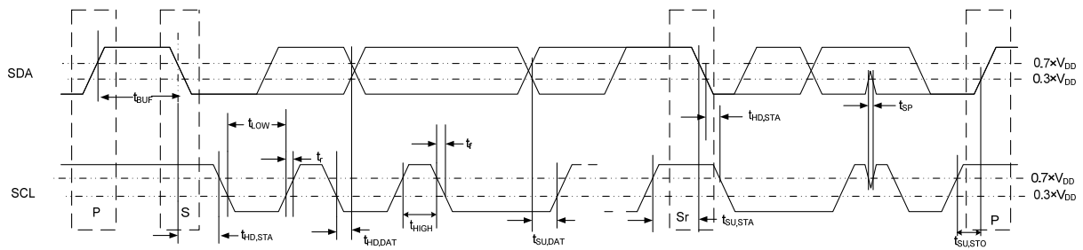
Figure 1. Definition of timing on the I²C-bus
