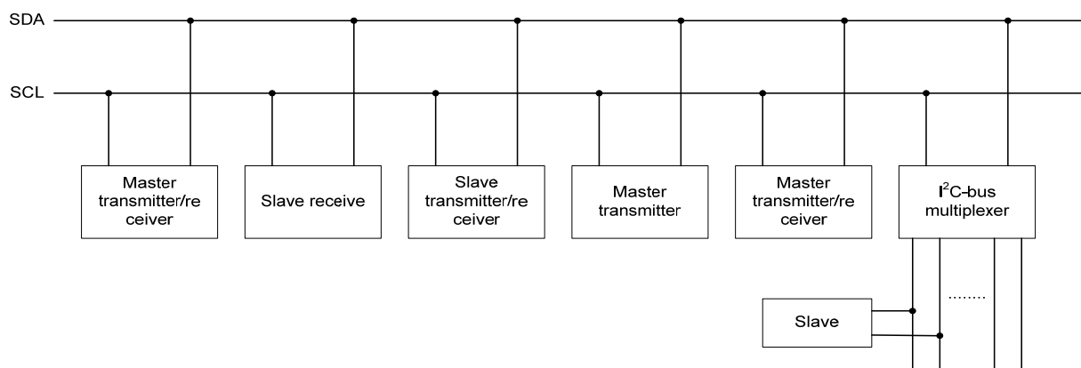
Figure 14. System configuration
