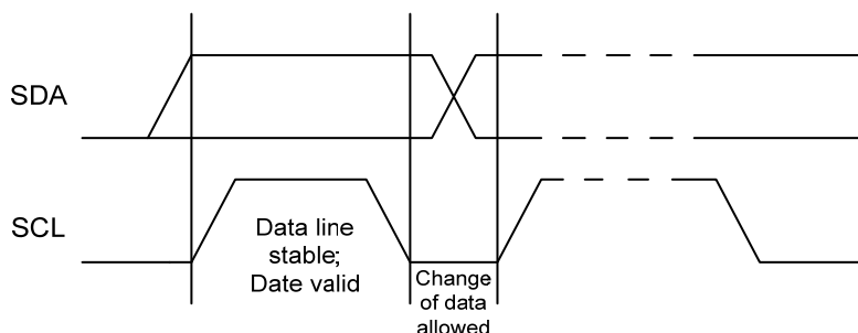
Figure 12. Bit transfer
