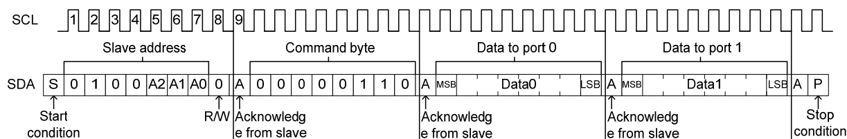
Figure 8. Write to configuration registers
