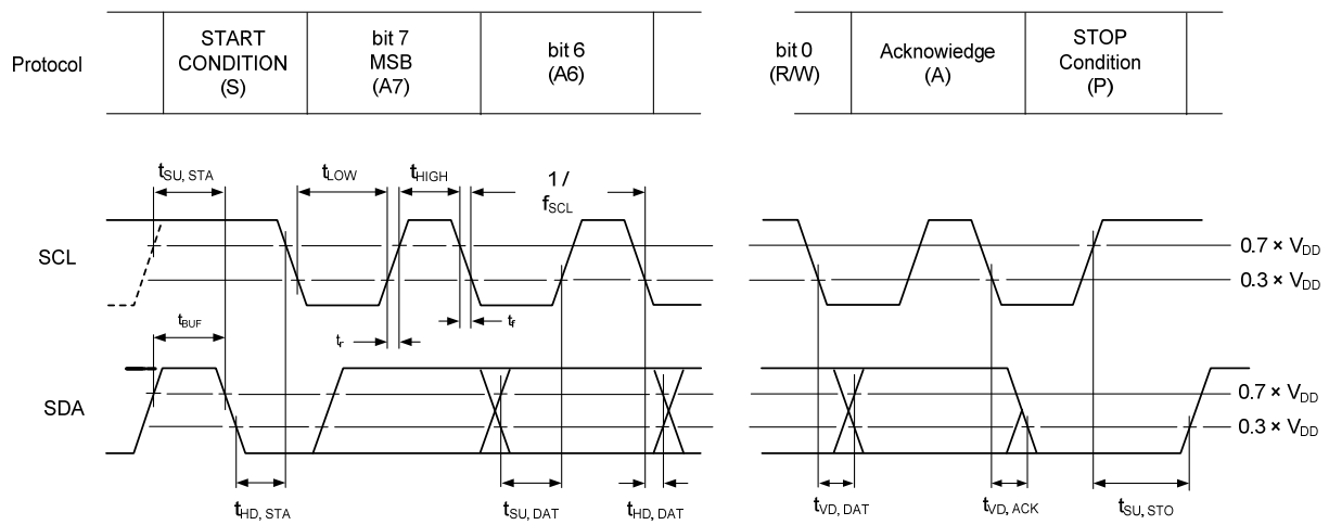
Figure 1. Definition of timing on the I²C-bus
