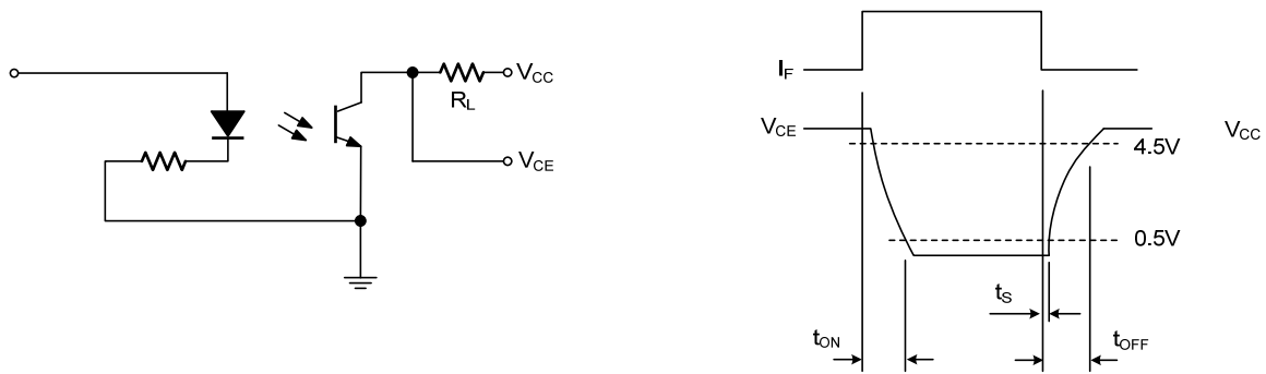
Test Circuit for Response Time
