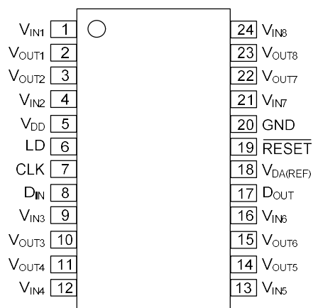
SOP-24 / SSOP-24N
